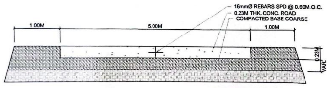
CROSS SECTION OF CONCRETE ROAD @ 5.00 M. WIDE SCALE: NTS
