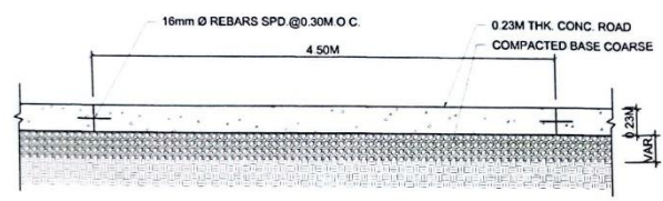
LONGITUDINAL SECTION OF CONCRETE ROAD SCALE: NTS
