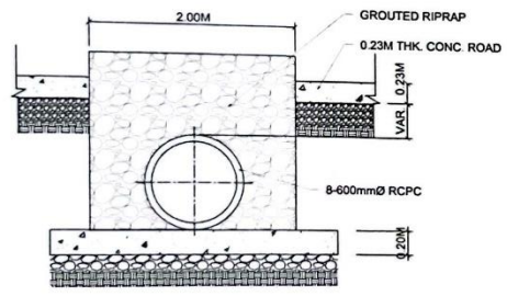
DETAIL OF HEADWALL & 600 MM Ø RCPC SCALE: NTS
