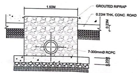
DETAIL OF HEADWALL & 300 MM Ø RCPC SCALE: NTS
