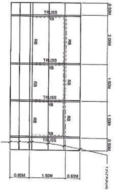
ROOF FRAMING PLAN SCALE: 1/10
