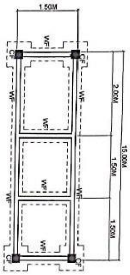
FOUNDATION PLAN SCALE: 1/10
