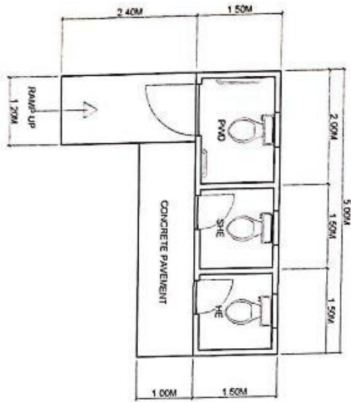
○ FLOOR PLAN SCALE
